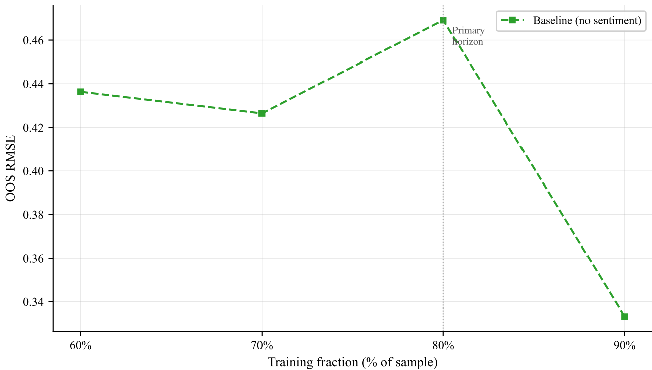
OOS RMSE by Training-Fraction Threshold -- Spec 4e Level Regression (top 4 combos)
